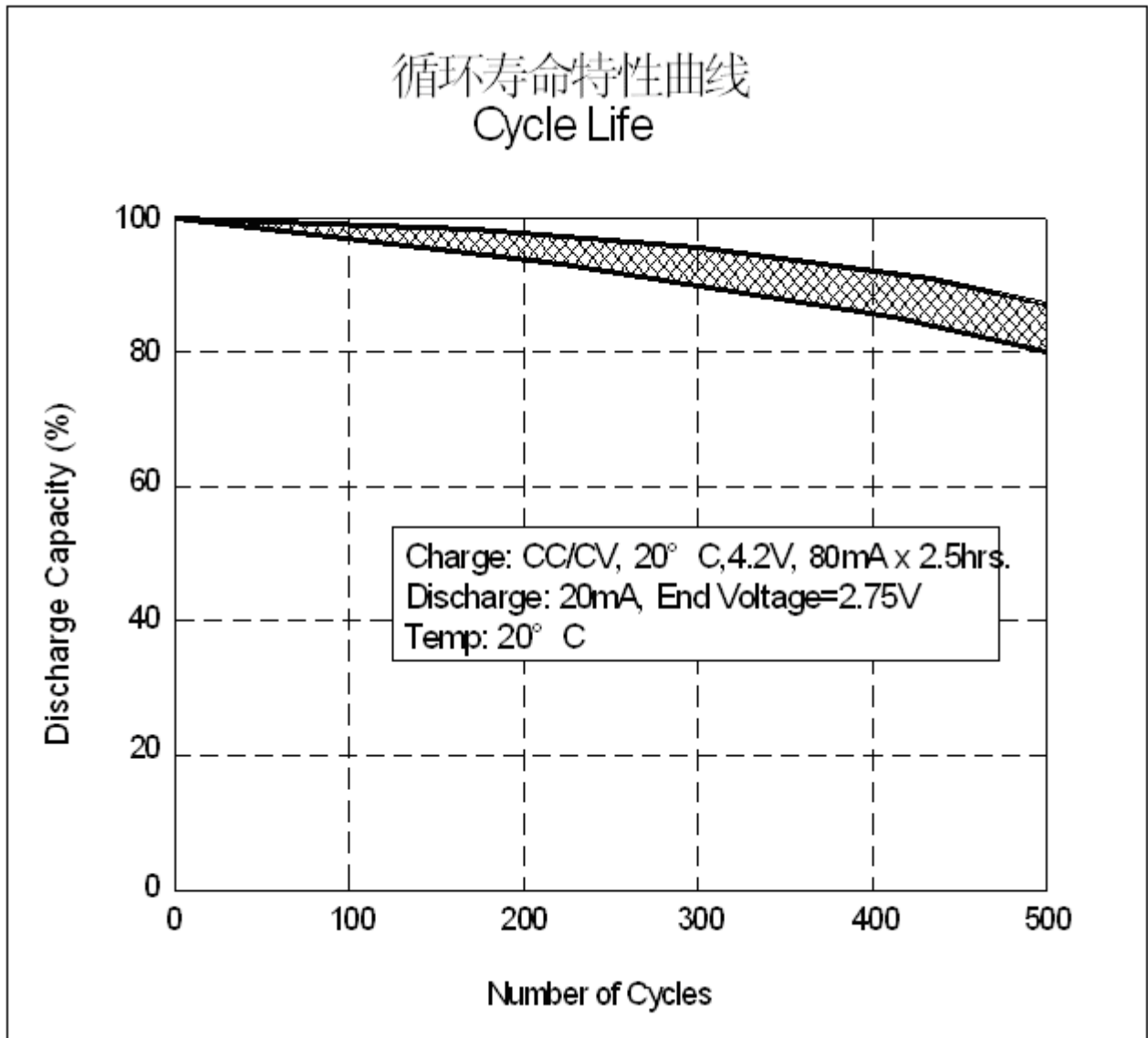
Fig. 5 Cycle Life Chart
